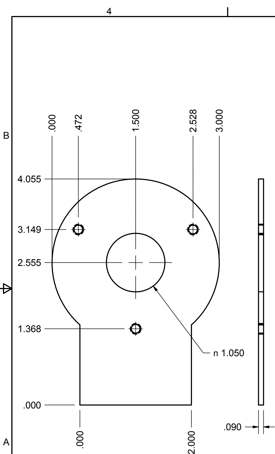
KNEE HINGE - LOWER SCALE 1 : 1
